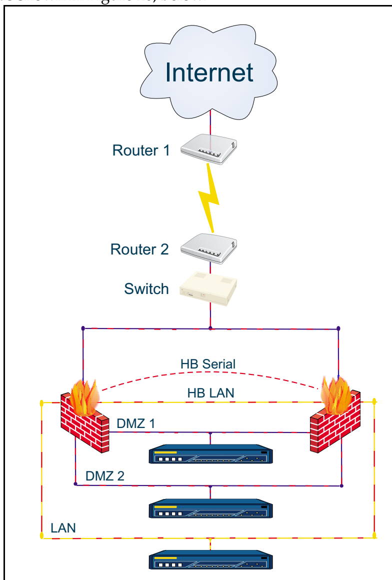
FIGURE 20: High-Availability Heart-beat configuration
