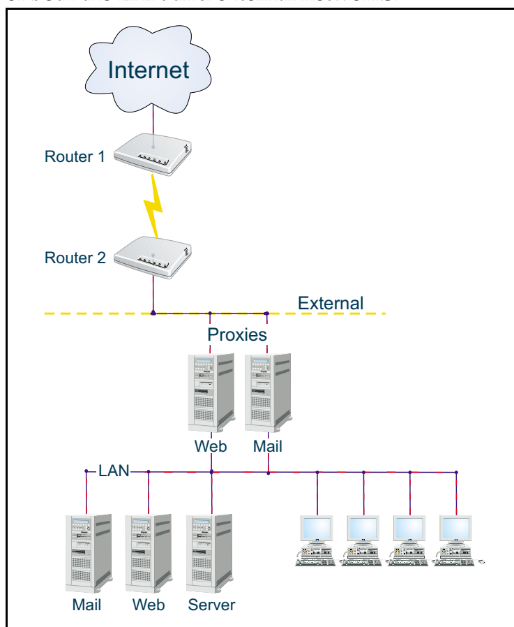
FIGURE 16: Multi-Homed Proxies
