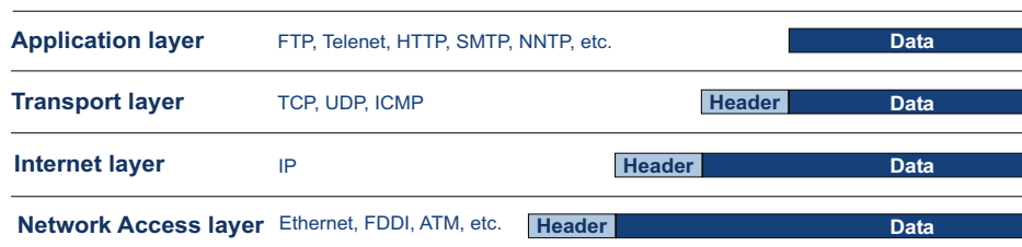
FIGURE 51: Data encapsulation
