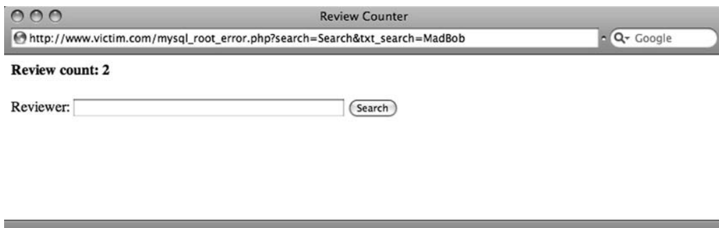
Figure 5.6 Query for “MadBob” Returning a Count of Two Reviews, Used As TRUE Inference
